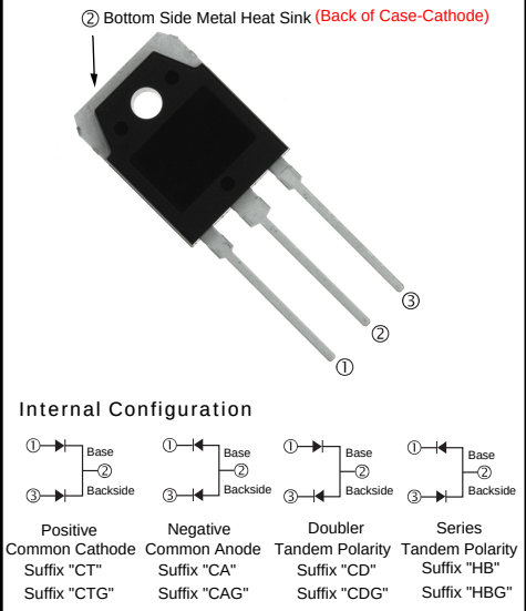
TO-3PN/TO-3PB-SQ
