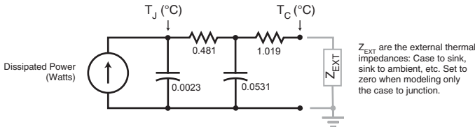
FIGURE 1b, TRANSIENT THERMAL IMPEDANCE MODEL
