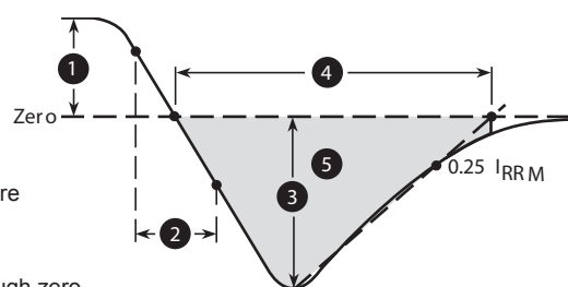
Figure 10. Diode Reverse Recovery Waveform Definition
