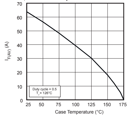
FIGURE 7, Maximum Average Forward Current vs. Case Temperature
