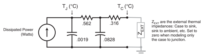
FIGURE 1b. TRANSIENT THERMAL IMPEDANCE MODEL
