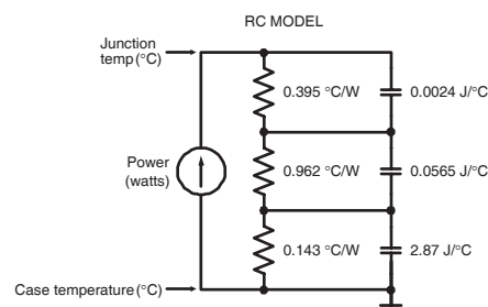
FIGURE 1b. TRANSIENT THERMAL IMPEDANCE MODEL
