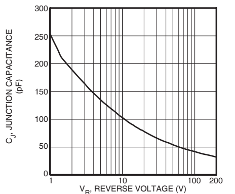
Figure 8. Junction Capacitance vs. Reverse Voltage
