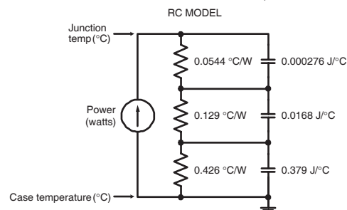
FIGURE 1b. TRANSIENT THERMAL IMPEDANCE MODEL
