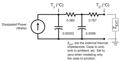
FIGURE 1b, TRANSIENT THERMAL IMPEDANCE MODEL
