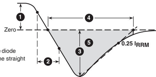
Figure 10, Diode Reverse Recovery Waveform and Definitions
